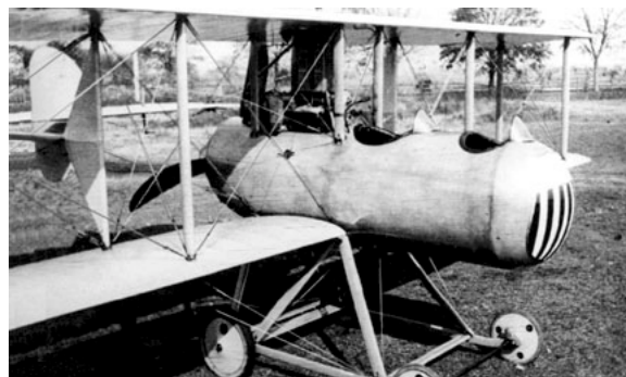
Figure 3. Photograph of the KB-1 Continental Pusher.
